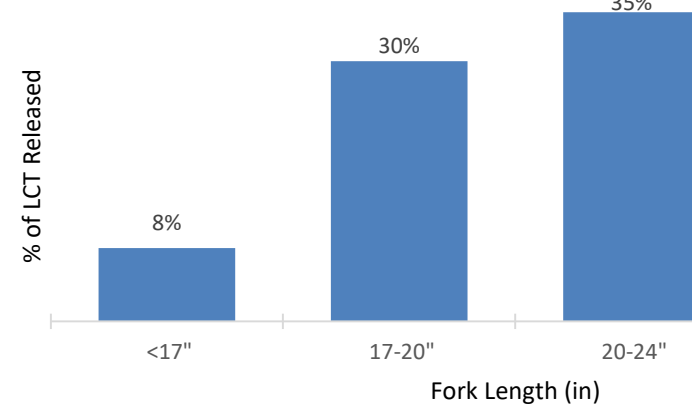
Size Distribution of Released LCT Reported by Boat Methods
